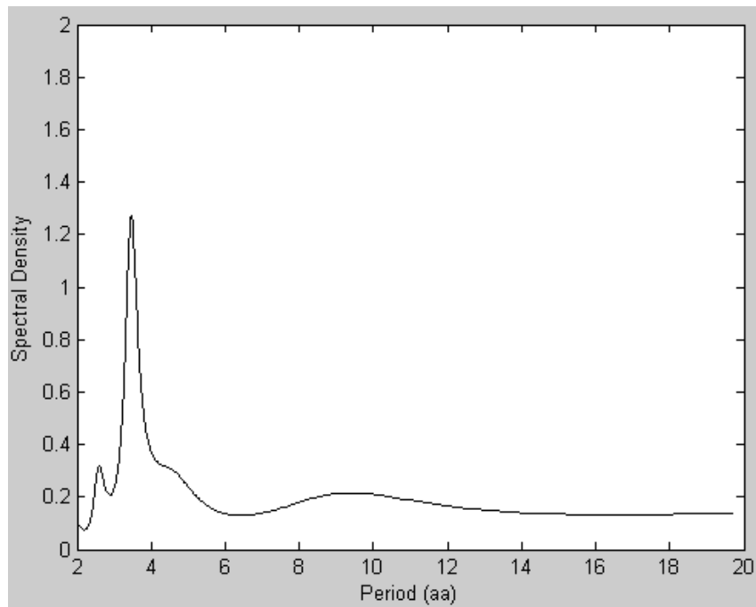
Fig.5 Spectral density plot of Factor II variances profile produced by Burg method.
