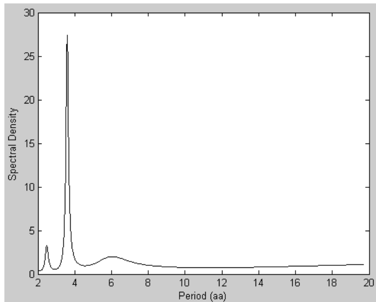
Fig.1 Spectral density plot of entropy profile produced by Burg method.
