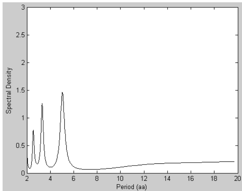
Fig.8 Spectral density plot of Factor IV means profile produced by Burg method.
