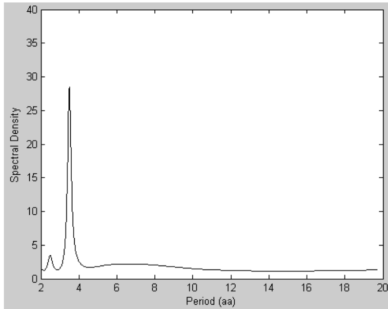
Fig.11 Spectral density plot of Factor V variances profile produced by Burg method.
