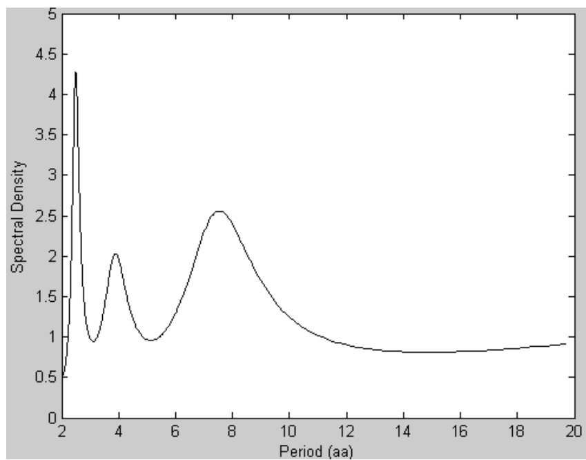
Fig.6 Spectral density plot of Factor III means profile produced by Burg method.
