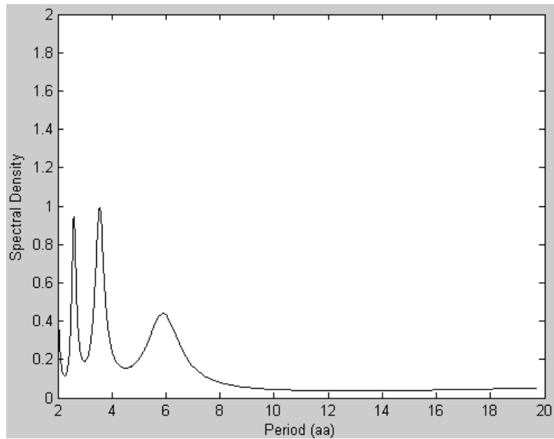
Fig.3 Spectral density plot of Factor I variances profile produced by Burg method.
