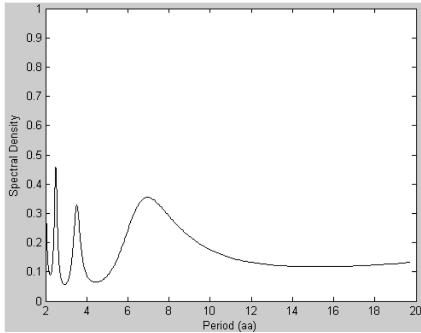
Fig.9 Spectral density plot of Factor IV variances profile produced by Burg method.
