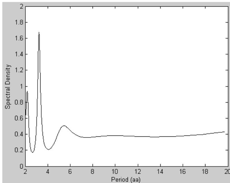
Fig.4 Spectral density plot of Factor II means profile produced by Burg method.
