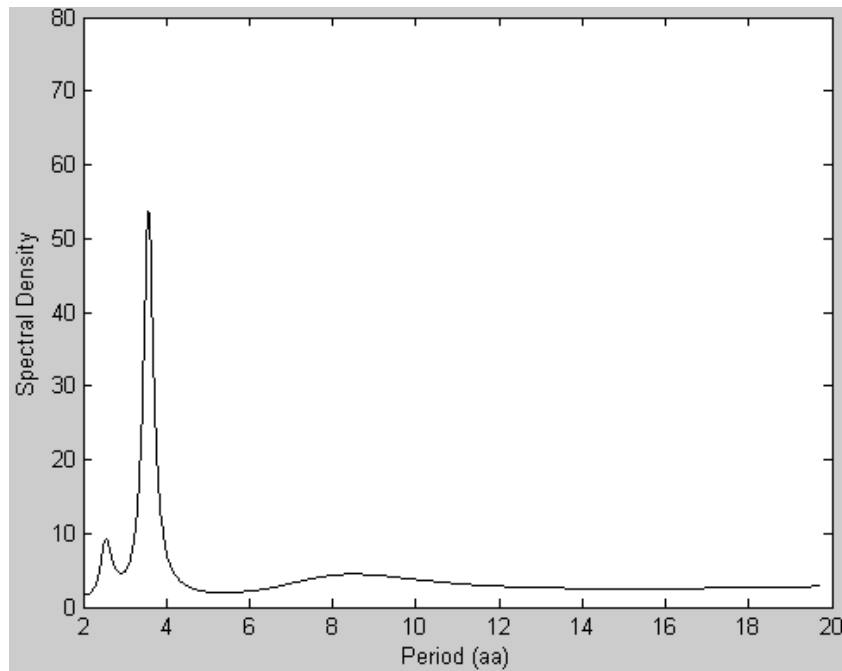
Fig.7 Spectral density plot of Factor III variances profile produced by Burg method.
