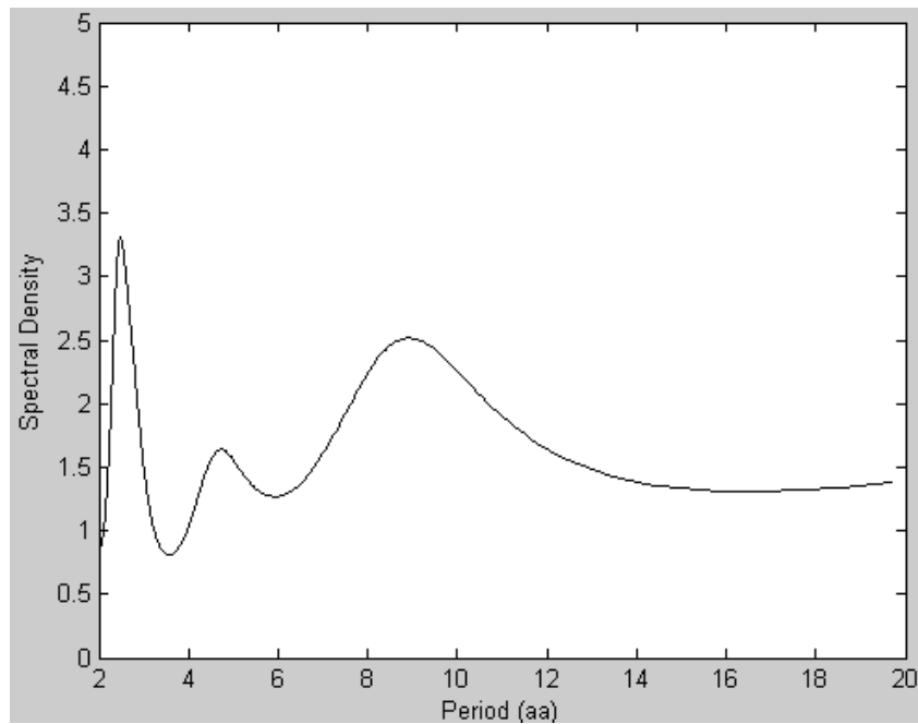
Fig.10 Spectral density plot of Factor V means profile produced by Burg method.
